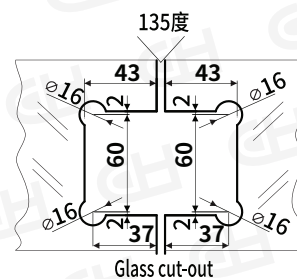
Glass cut-out
