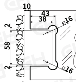
Glass cut-out
