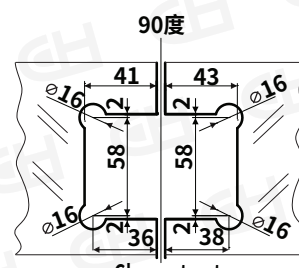
Glass cut-out
