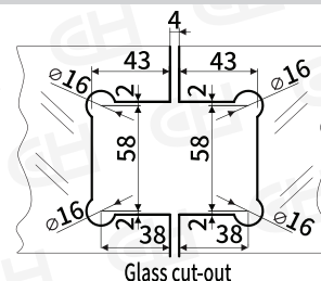
Glass cut-out
