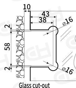
Glass cut-out
