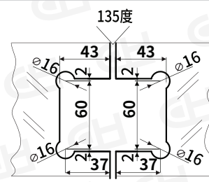
Glass cut-out
