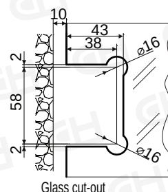
Glass cut-out
