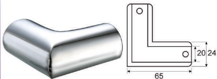
CH-III8-4 (管對管90度)
